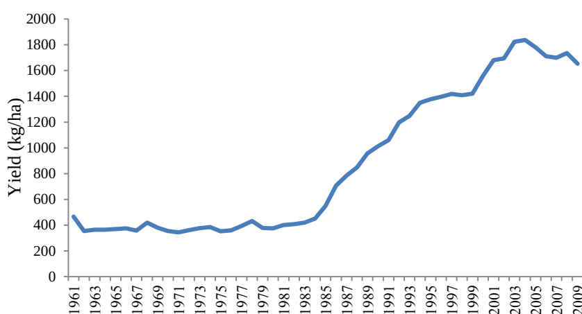
Figure 1-1 Evolution of rubber yield in Southern Thailand
