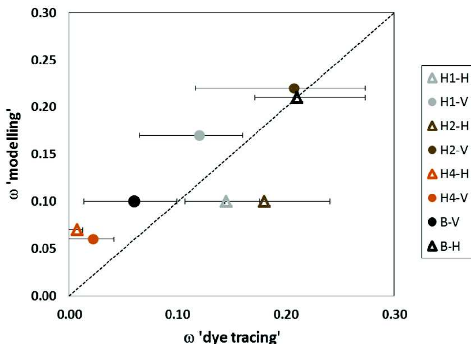
Figure 4.1-6: Correspondence of simulated and measured effective macroporosity fractions. The error bars represent the minimal and maximal \omega among the 7 cross-sections of a given soil column.
