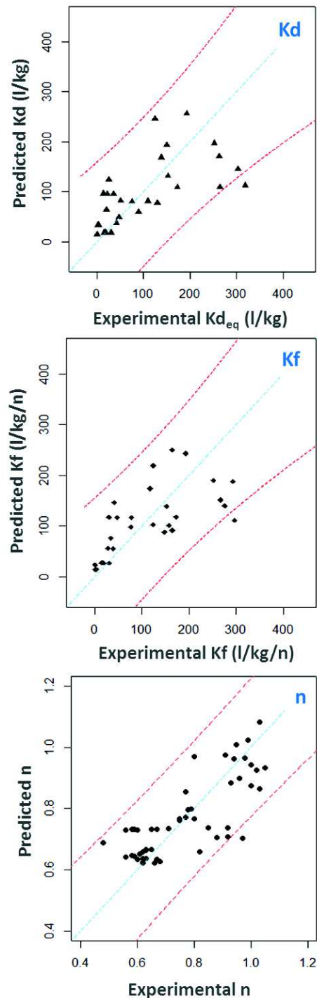
Figure C.2: Multiple regression analysis of the sorption coefficients ( K_d , K_f , n ) and soil properties. The sorption coefficients predicted from the pedotransfer functions presented in Table 6 were plotted against the sorption coefficients ( K_f, n ) fitted from the experimental data and for K_{d_{eq}} against the linearized sorption coefficients.
