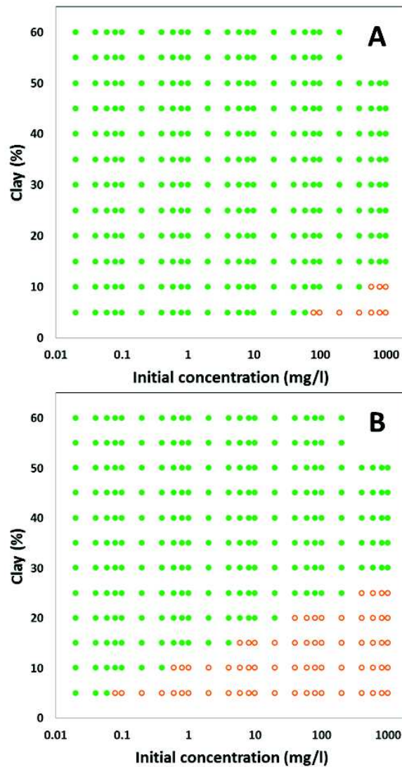
Figure C.4: Linearity range of sorption isotherms in relation to the clay content and initial glyphosate concentrations in the liquid phase. Plain green dots represent 0.9 < n < 1.05 , and empty orange dots represent n values lower than 0.9 (bottom right). A: n values were calculated from equation 4 with a solid-to-liquid ratio of 1:1 (g/ml). B: n values were calculated from Equation 4 with a solid-to-liquid ratio of 1:20 (g/ml). Note that for a solid-to-liquid ratio of 1:1, the saturation of sorption sites occurs at initial concentration higher than 100 mg/l for clay content varying between 0 and 10%, whereas for the 1:20 ratio, the saturation for the same clay content starts at initial concentrations of approximately 0.1 mg/l.
