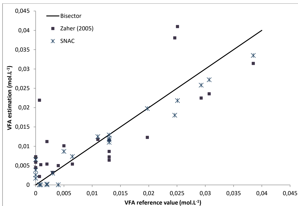
Figure 21: Comparison of VFA estimation using buffer capacity, Zaher (2005), or buffer capacity coupled to buffer conductivity (SNAC)
