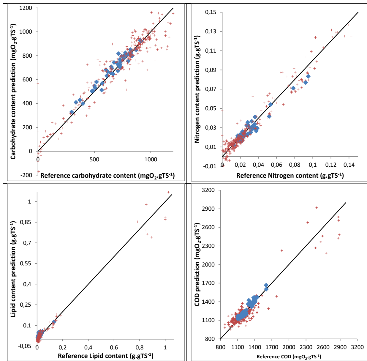
Figure 39: Prediction performances of carbohydrate, nitrogen and lipid contents and COD, respectively on the top left, top right, bottom left and bottom right. The blue squares (●) represent the prediction of the independent validation set whereas the red crosses (+) represent the estimation of the calibration set. The line represents the bisector between reference and predicted values.
