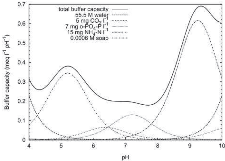
Figure 12: Buffer capacity curve for a complex aqueous system containing 5mg CO 2 .L -1 , 7 mg o-PO 4 -P.L -1 , 15 mg NH 4 + -N.L -1 and 0.6 meq.L -1 of an unspecified soap (Van Vooren 2000).
