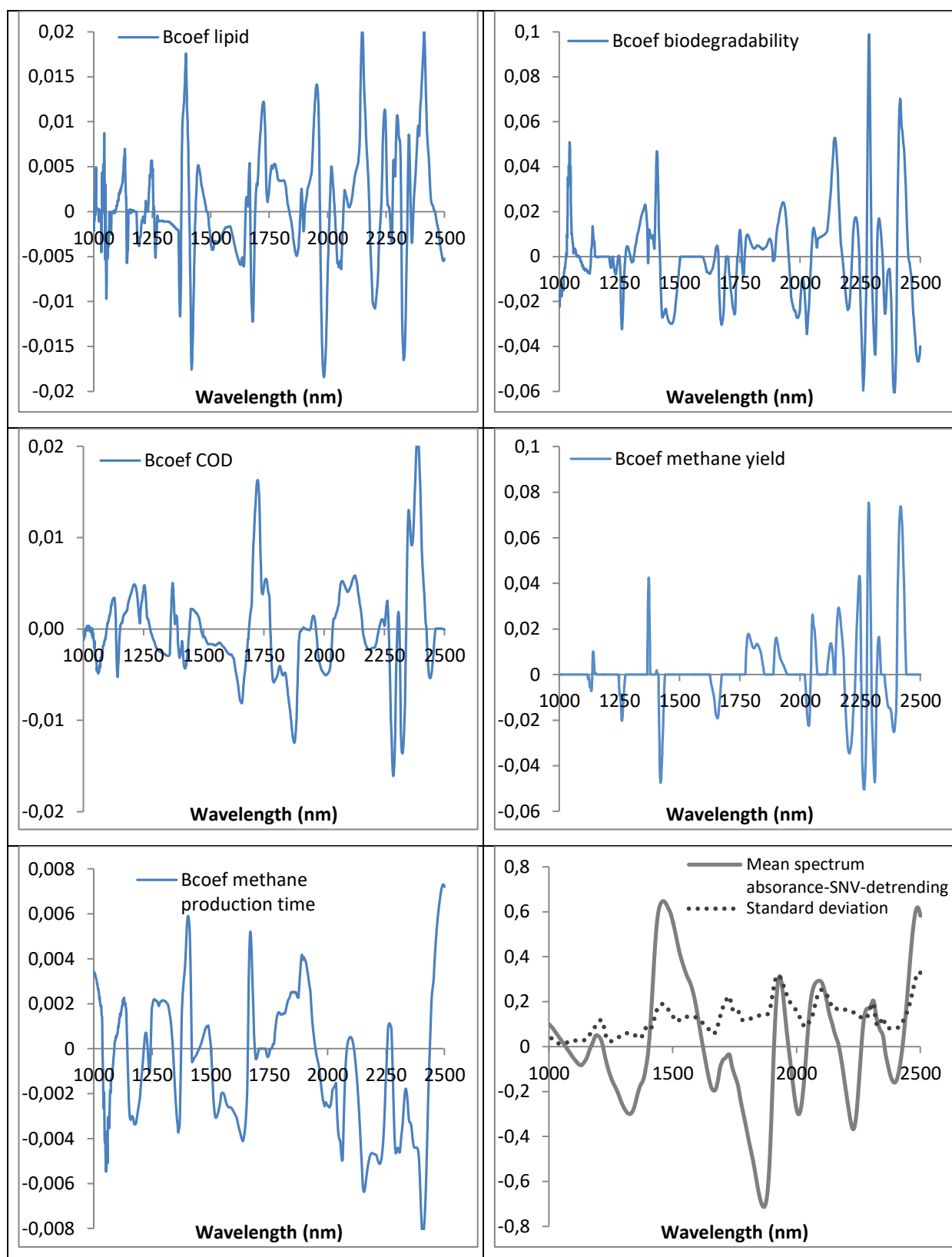
Figure 47: b coefficients (Bcoef) of carbohydrate, protein and lipid contents, biodegradability, COD, methane yield and methane production time prediction from spectra pretreated by absorbance/SNV/detrending
